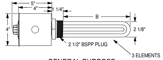
GENERAL PURPOSE WITH THERMOSTAT 3 ELEMENTS
