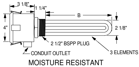
MOISTURE RESISTANT 3 ELEMENTS
