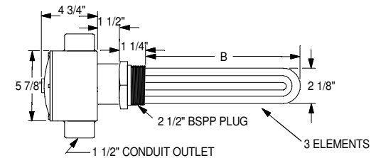
EXPLOSION RESISTANT WITH THERMOSTAT 3 ELEMENTS
