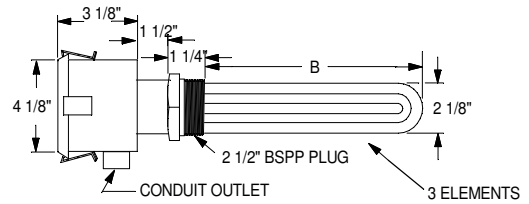
MOISTURE RESISTANT WITH THERMOSTAT 3 ELEMENTS
