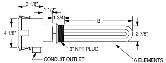
MOISTURE RESISTANT WITH THERMOSTAT 6 ELEMENTS
