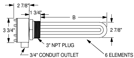
EXPLOSION RESISTANT 6 ELEMENTS
