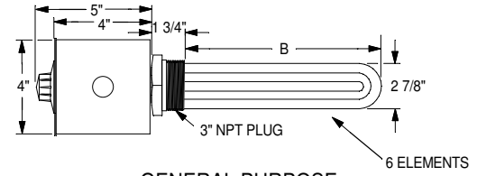
GENERAL PURPOSE WITH THERMOSTAT 6 ELEMENTS
