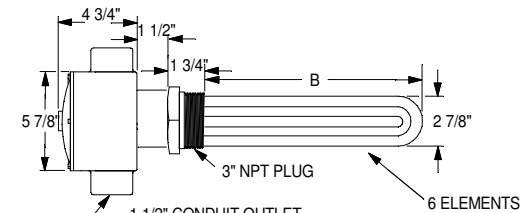
EXPLOSION RESISTANT WITH THERMOSTAT 6 ELEMENTS
