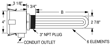
MOISTURE RESISTANT 6 ELEMENTS
